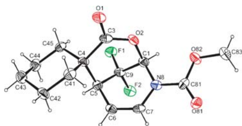
Fig. 1 X-Ray crystal structure of compound 11b . Ellipsoids are drawn at the 30% probability level.
