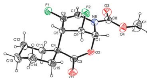
Fig. 2 X-Ray crystal structure of compound 12b . Ellipsoids are drawn at the 30% probability level.
